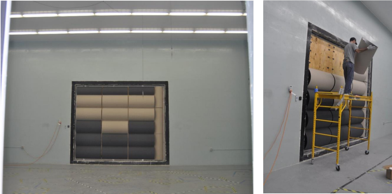
Photos: Curve Diffusor Low-Frequency Absorption test, NWAA Labs, 18 August 2015
